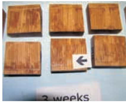
The arrow is pointing to some shiny epoxy found in a three-week 105/205 sample. Close examination showed that it was not a cohesive failure-both matching areas were shiny, which indicates a void. This sample was not included in the average.
