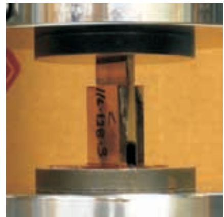
Below—A double lap shear test in progress. The double lap shear test is more accurate than the single lap shear test.
