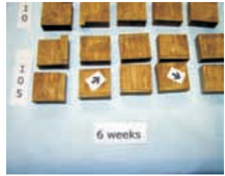
The arrows are again pointing to shiny glue areas indicating a void. The area of the void was large enough on the #4 sample (l-r) that it too was excluded from the average. The effective area of the void on #2 was deemed insignificant and so it was included in the average. Interestingly, even though the average strength of this set of 105/205 samples was 729 psi, there was still no cohesive failure of the glue line.
