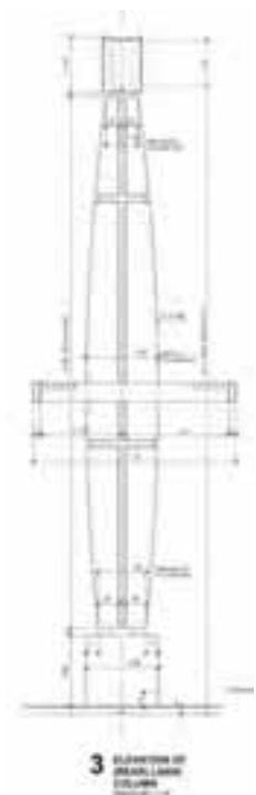
Architect’s elevation of the 18' rear columns.
