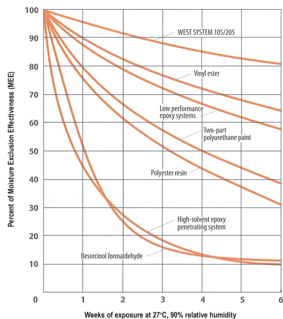
Adding solvent comprises the moisture resistance of cured epoxy
