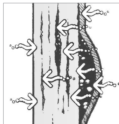
Figure 1-6 Accumulating fluid creates enough hydraulic pressure in the voids between the gelcoat and laminate to result in a gelcoat blister.
