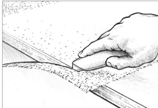
Figure 6-13 Trim excess cloth when the epoxy reaches its initial cure phase. The wet-out cloth will be dry but flexible and will trim easily with a sharp utility knife.
